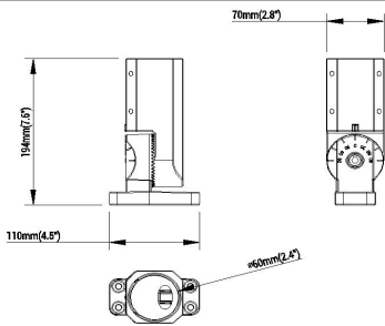
Ø60mm Slipfitter
