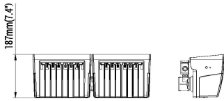
Wall Mount
