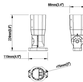
Ø76mm Slipfitter
