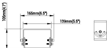
Ø60mm Slipfitter
